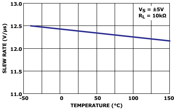
FIGURE 11. SLEW RATE vs TEMPERATURE
