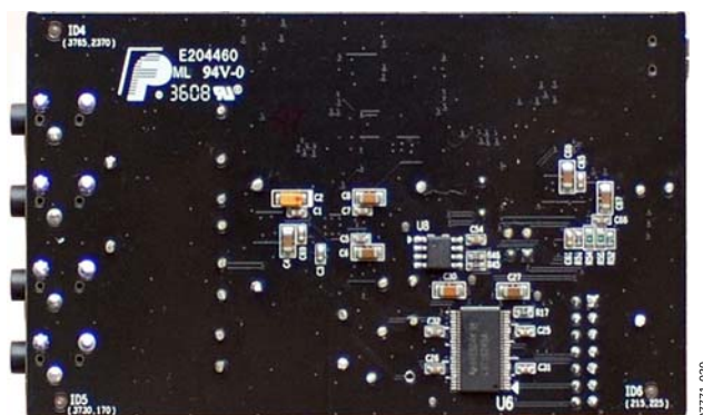
Figure 2. Bottom View of the SSM2603 Evaluation Board
