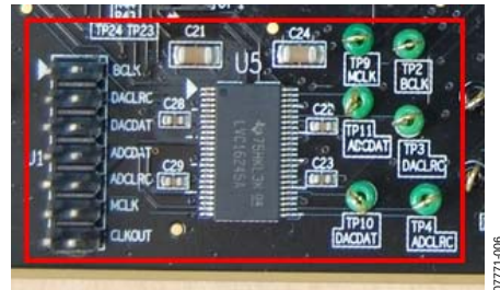
Figure 7. General-Purpose Digital Audio Interface and Buffer
