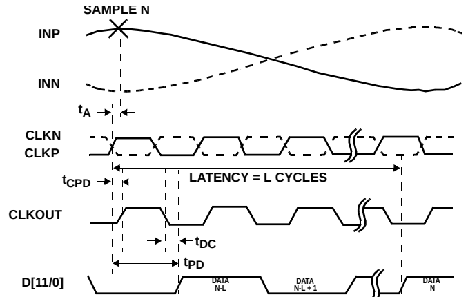
FIGURE 2B. SDR
