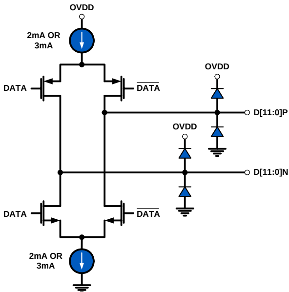
FIGURE 45. LVDS OUTPUTS
