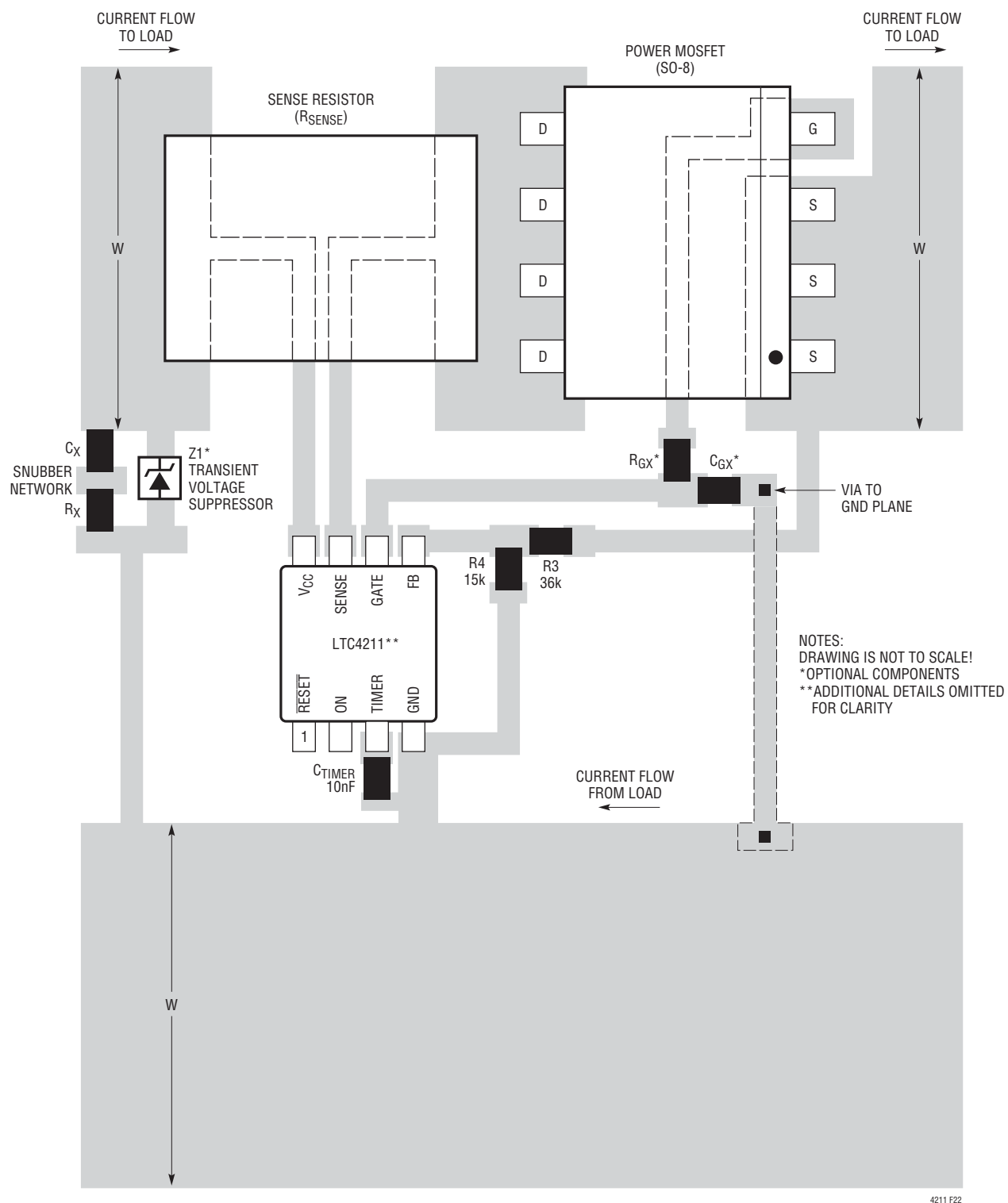
Figure 22. Recommended Layout for LTC4211 Protection Devices, R_{\text{SENSE}} , Power MOSFET and Feedback Network
