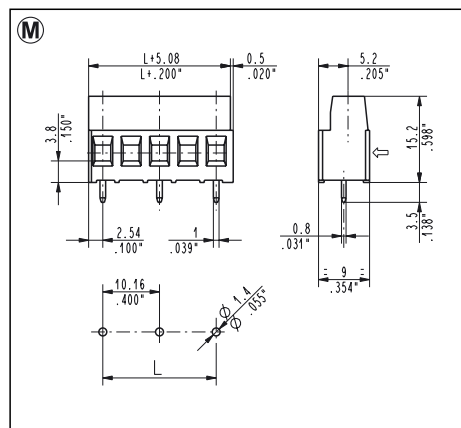
MSM_006 Straight, Side Entry 10.16 mm / .400" Pitch Weight per pole: 1.77 g
