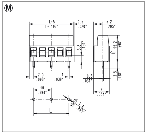
MSM_002 - 000T 10 mm / .394" Pitch
