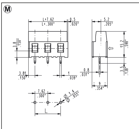
MSM_007 Straight, Side Entry 7.62 mm / .300" Pitch Weight per pole: 1.75 g
