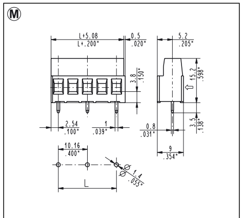
MSM_006 - 000T 10.16 mm / .400" Pitch
