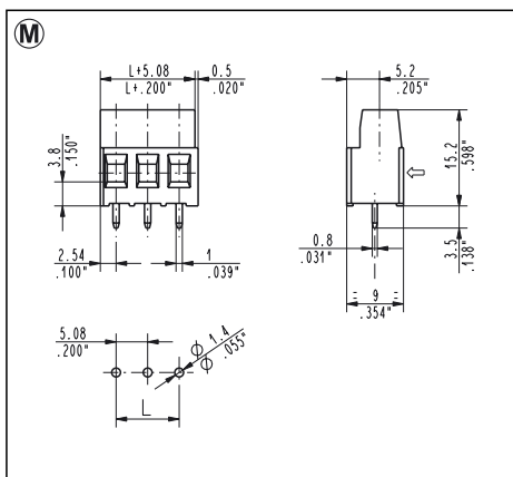
MSM_005 Straight, Side Entry 5.08 mm / .200" Pitch Weight per pole: 1.56 g
