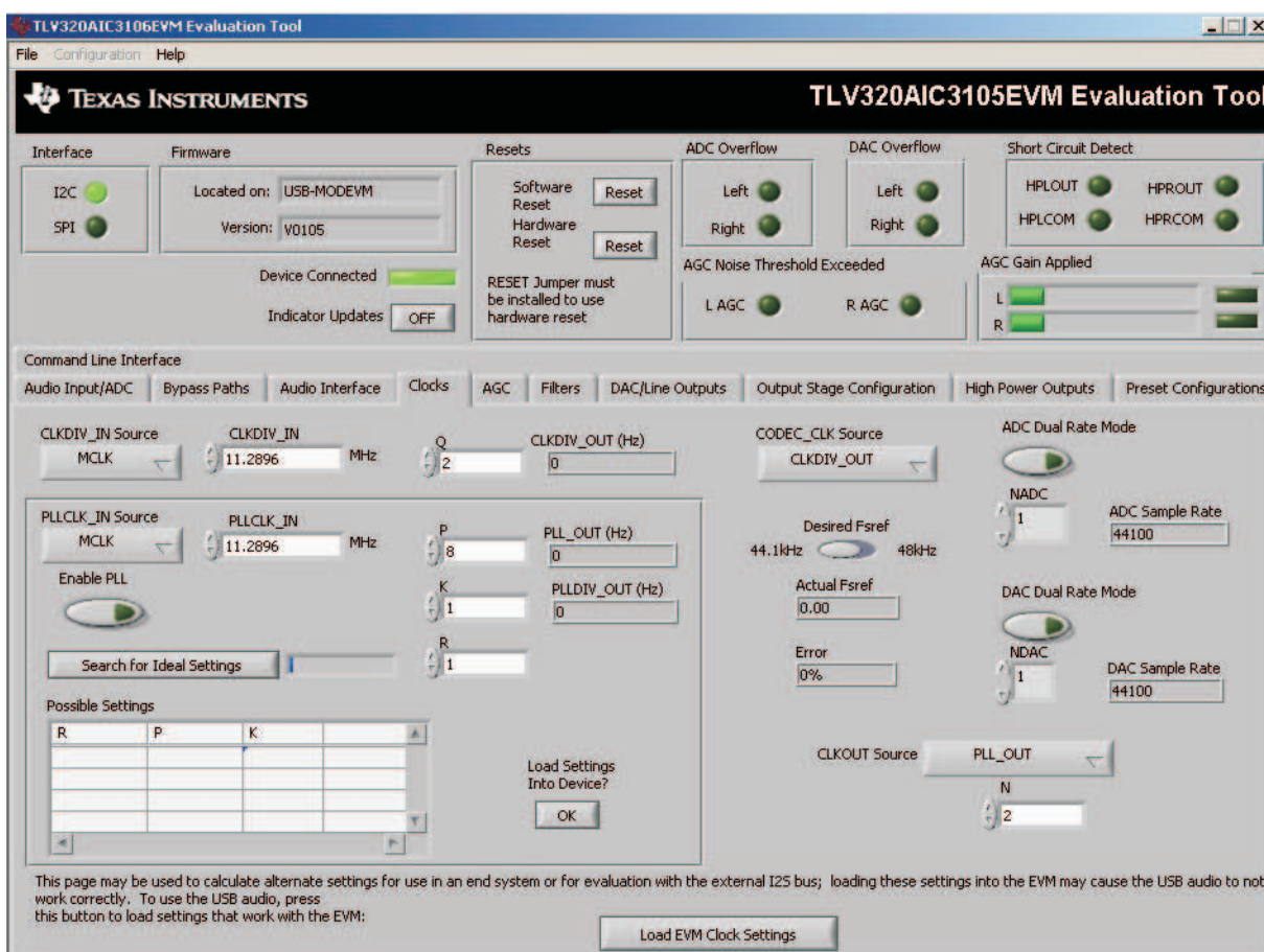
Figure 8. Clocks Tab
