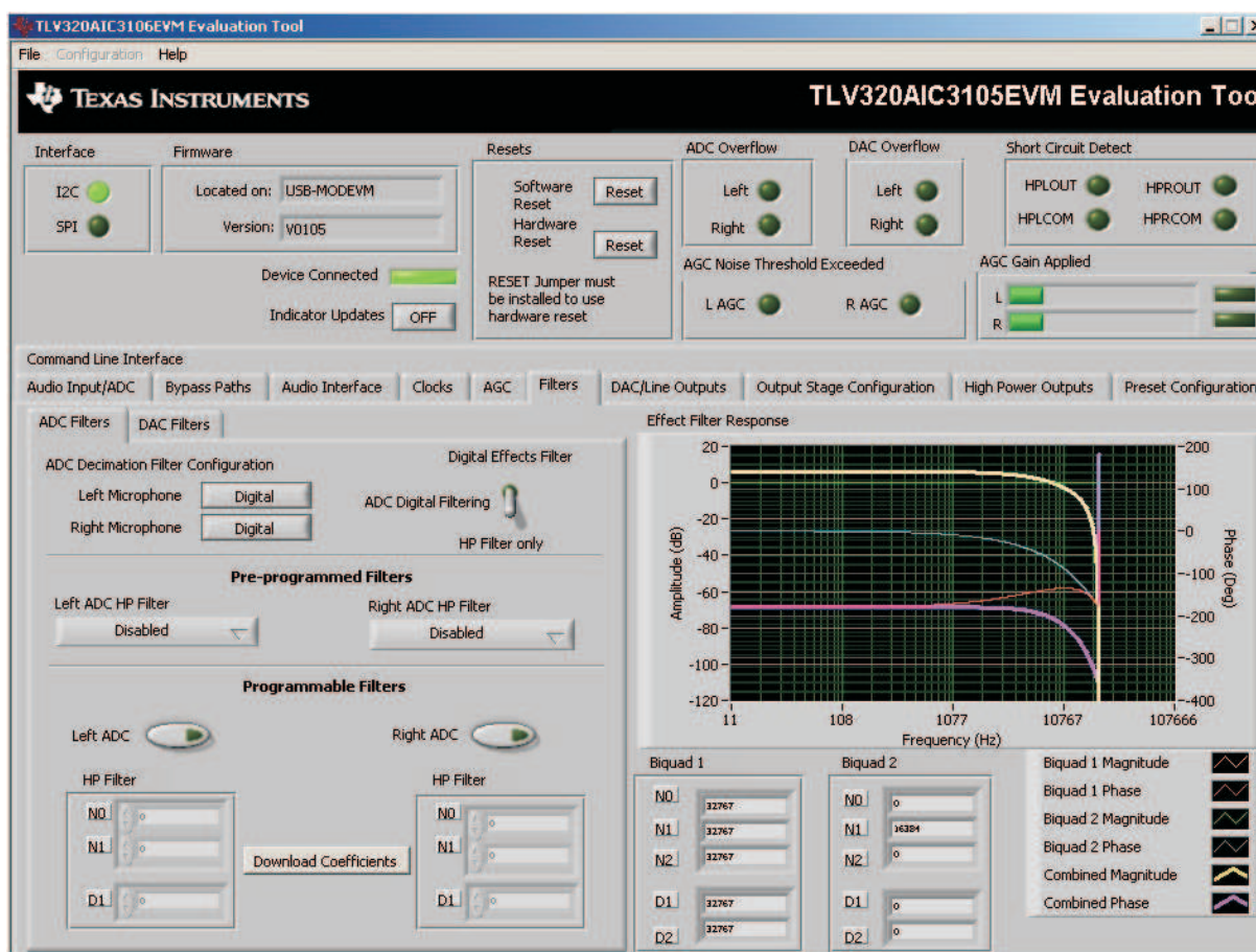
Figure 12. Filters Tab
