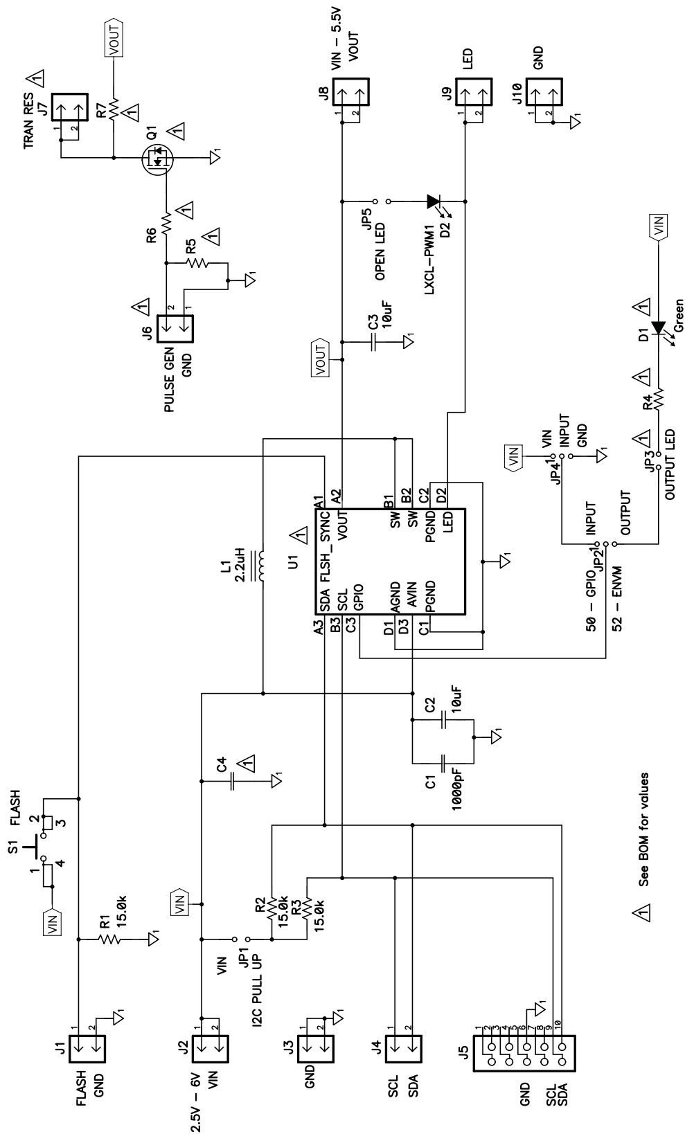
Figure 14. TPS61050/2EVM-269 Schematic
