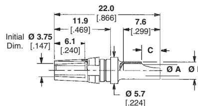
Female, Cable
