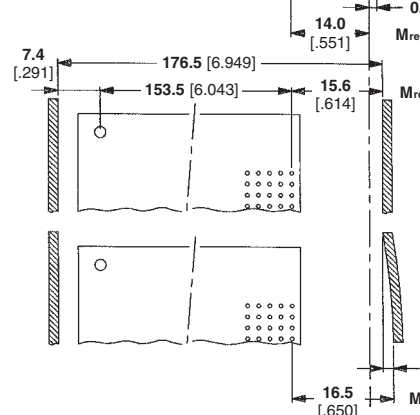
Subrack tolerances
