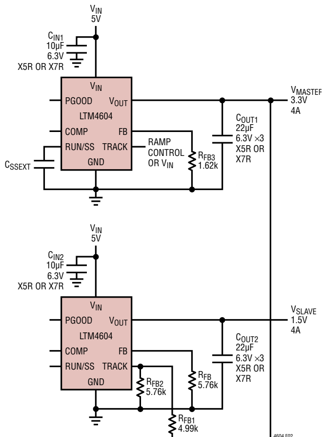
Figure 2. Dual Outputs (3.3V and 1.5V) with Tracking
