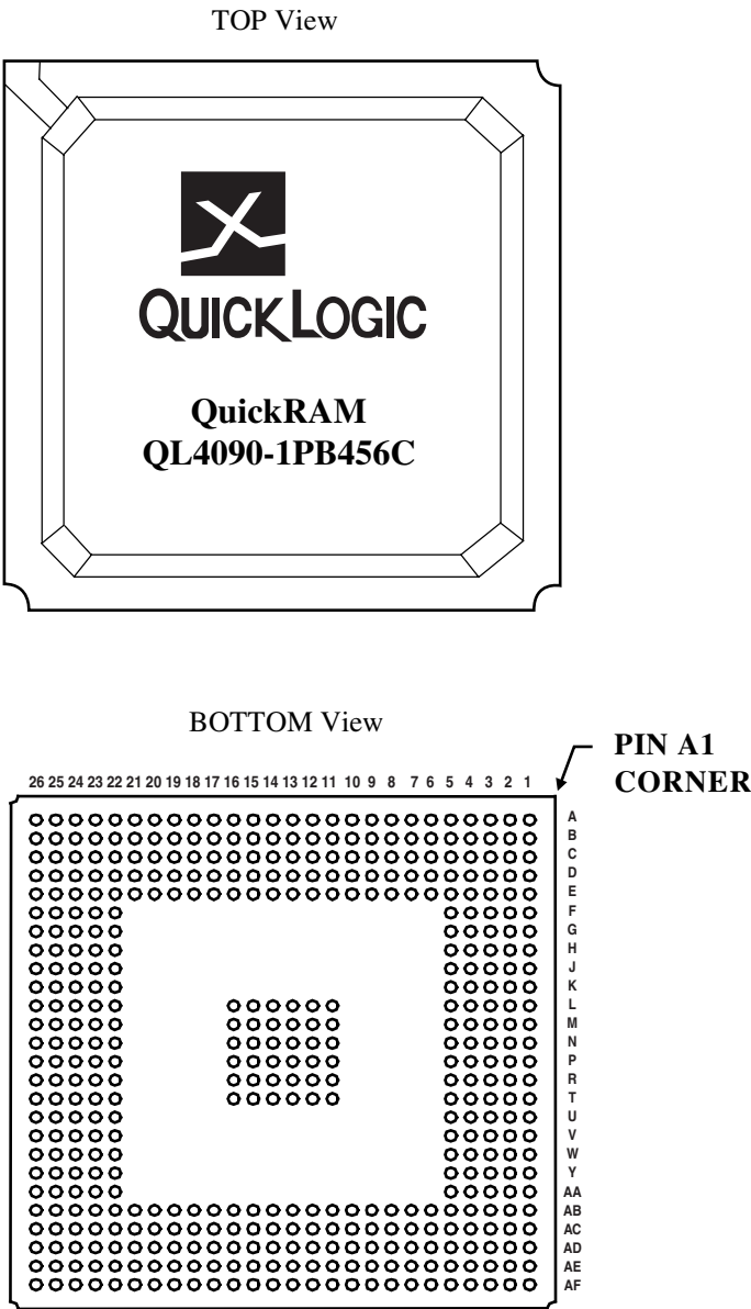
Figure 13: 456 PBGA Pinout Diagram
