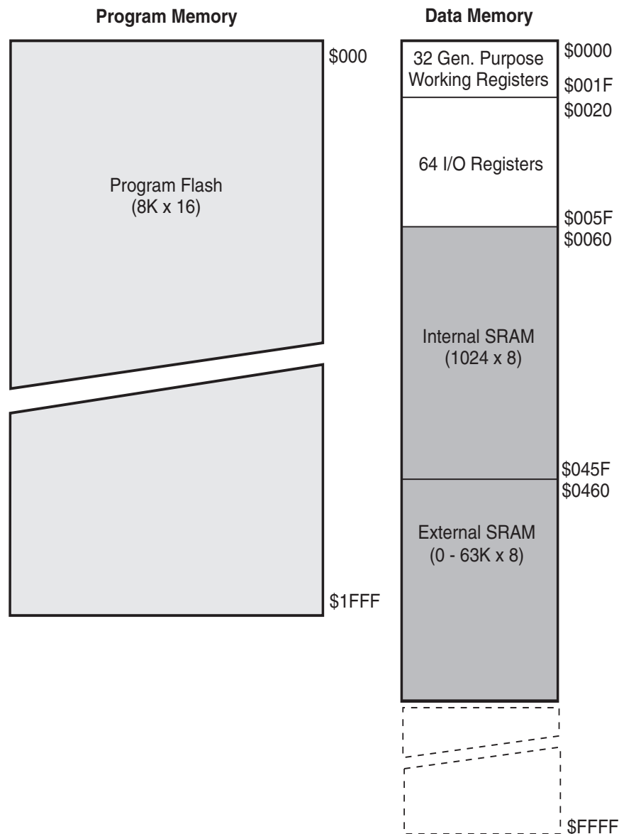
Figure 5. Memory Maps
