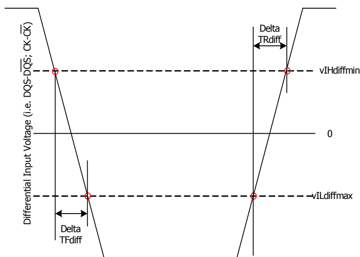
Differential Input Slew Rate Definition for DQS, \overline{\text{DQS}} and CK, \overline{\text{CK}}
