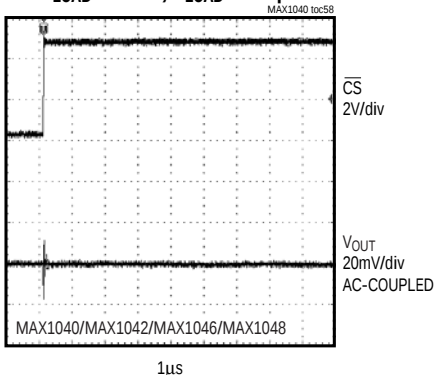
MAJOR CARRY TRANSITION RLOAD = 10kΩ, CLOAD = 100pF
