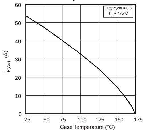
FIGURE 29, Maximum Average Forward Current vs. Case Temperature
