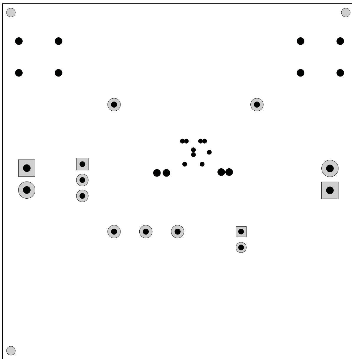
Figure 10. EVM Bottom-Side Layout
