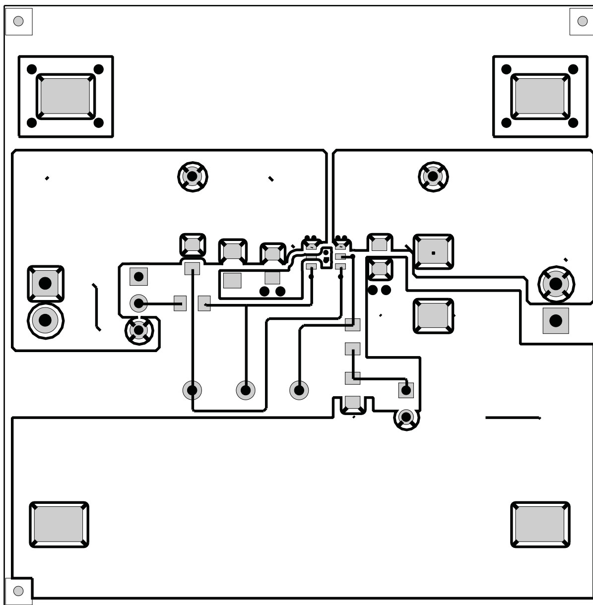
Figure 8. EVM Top-Side Layout
