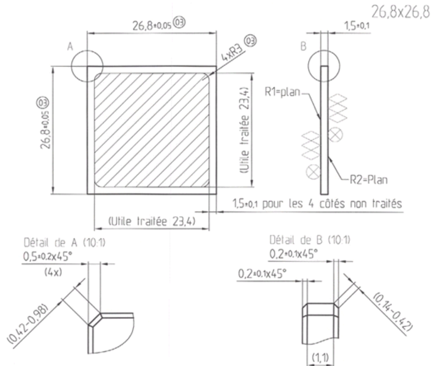
Figure 5. Glass Lid Dimensions
