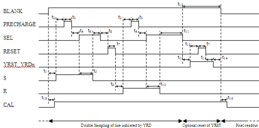
Figure 35. Destructive Readout Timing Diagram
