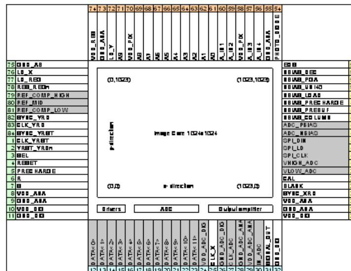
Figure 6. Pin Assignment
