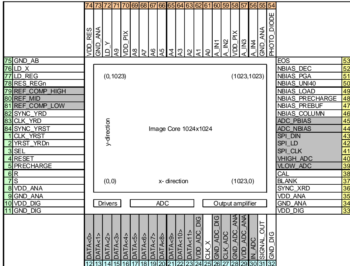
Figure 26. Pin Configuration
