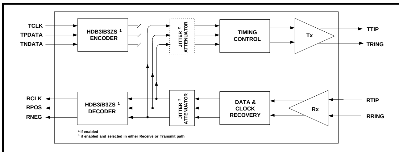
FIGURE 28. REMOTE LOOPBACK
