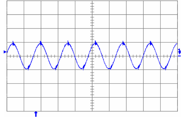
Fig. 2.5V.6: Output voltage ripple ( 20\text{ mV/div.} ) at full rated load current into a resistive load with external capacitance 100\text{ }\mu\text{F} ceramic + 1\text{ }\mu\text{F} ceramic and V_{in} = 5\text{ V} for V_{out} = 2.5\text{ V} . Time scale: 2\text{ }\mu\text{s/div.}
