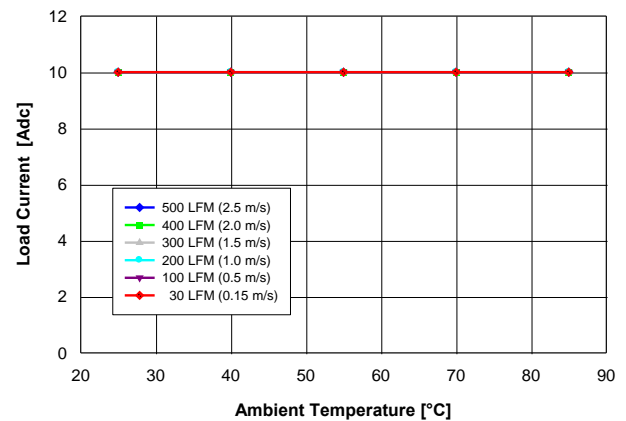
Fig. 1.2V.2: Available load current vs. ambient temperature and airflow rates for V_{out} = 1.2 V converter mounted horizontally with V_{in} = 5 V, and maximum MOSFET temperature \leq 120^\circ\text{C} .
