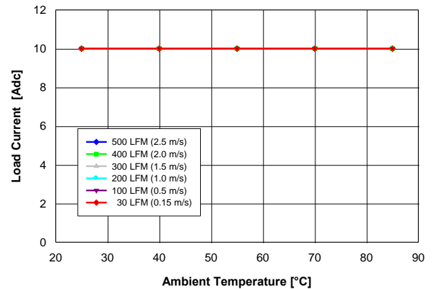
Fig. 2.5V.2: Available load current vs. ambient temperature and airflow rates for V_{out} = 2.5 V converter mounted horizontally with V_{in} = 5 V, and maximum MOSFET temperature \leq 120^\circ\text{C} .
