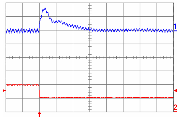
Fig. 2.0V.8: Output voltage response for V_{out} = 2.0 V to negative load current step change from 10 A to 5 A with slew rate of -5\ \text{A}/\mu\text{s} at V_{in} = 5 V. Top trace: output voltage (100 mV/div.); Bottom trace: load current (5 A/div.). C_o = 100\ \mu\text{F} ceramic + 1\ \mu\text{F} ceramic. Time scale: 20 µs/div.
