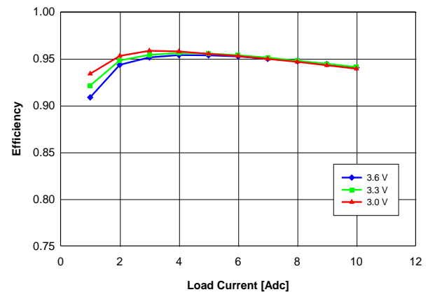
Fig. 2.5V.4: Efficiency vs. load current and input voltage for V_{out} = 2.5 V converter mounted vertically with air flowing at a rate of 200 LFM (1 m/s) and T_a = 25^\circ\text{C} .
