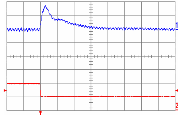
Fig. 1.5V.8: Output voltage response for V_{out} = 1.5 V to negative load current step change from 10 A to 5 A with slew rate of -5 \text{ A}/\mu\text{s} at V_{in} = 5 V. Top trace: output voltage (100 mV/div.); Bottom trace: load current (5 A/div.). C_o = 100 \mu\text{F} ceramic + 1 \mu\text{F} ceramic. Time scale: 20 \mu\text{s} /div.
