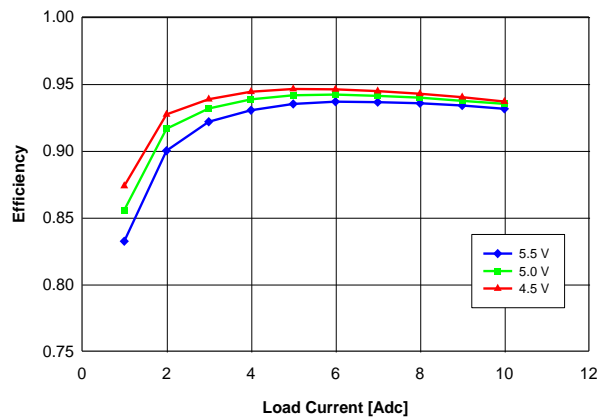
Fig. 2.5V.3: Efficiency vs. load current and input voltage for V_{out} = 2.5 V converter mounted vertically with air flowing at a rate of 200 LFM (1 m/s) and T_a = 25^\circ\text{C} .
