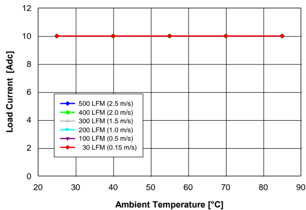
Fig. 1.2V.1: Available load current vs. ambient temperature and airflow rates for V_{out} = 1.2 V converter mounted vertically with V_{in} = 5 V, and maximum MOSFET temperature \leq 120^\circ\text{C} .
