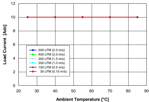
Fig. 2.5V.1: Available load current vs. ambient temperature and airflow rates for V_{out} = 2.5 V converter mounted vertically with V_{in} = 5 V, and maximum MOSFET temperature \leq 120^\circ\text{C} .
