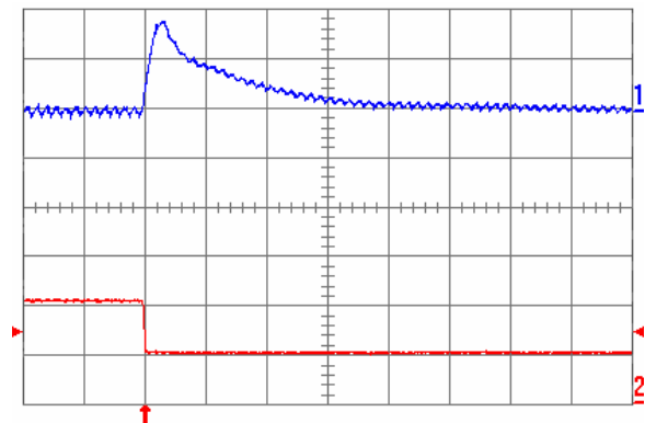
Fig. 1.2V.8: Output voltage response for V_{out} = 1.2 V to negative load current step change from 10 A to 5 A with slew rate of -5 A/ \mu s at V_{in} = 5 V. Top trace: output voltage (100 mV/div.); Bottom trace: load current (5 A/div.). C_o = 100 \mu F ceramic + 1 \mu F ceramic. Time scale: 20 \mu s/div.
