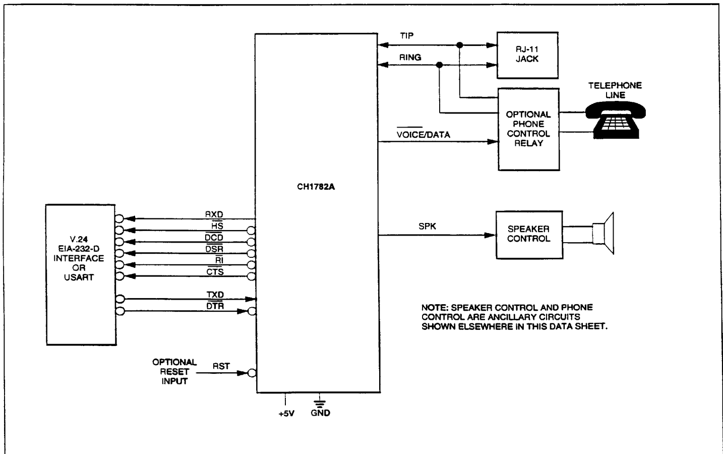
Figure 3a. CH1782A Application Diagram.
