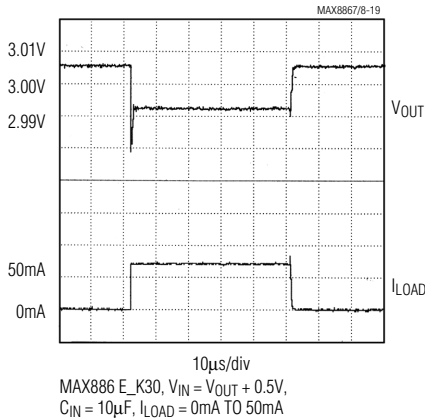
LOAD-TRANSIENT RESPONSE
