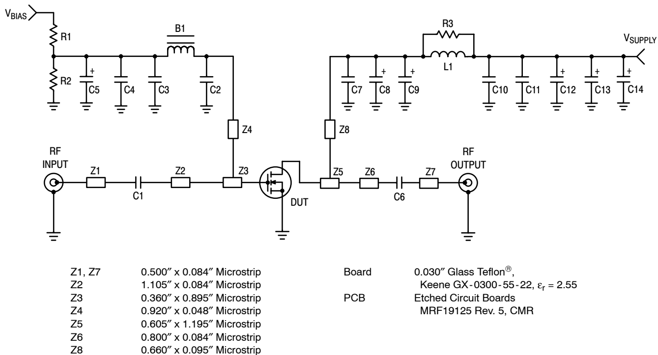
Figure 1. MRF19125R3(SR3) Test Circuit Schematic
