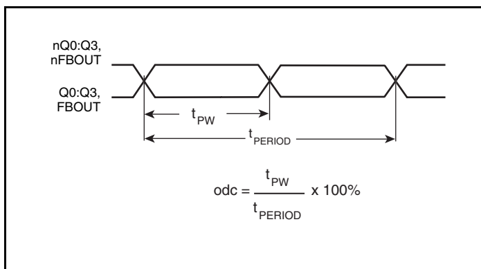
LVPECL/LVDS Output Duty Cycle/Pulse Width/Period
