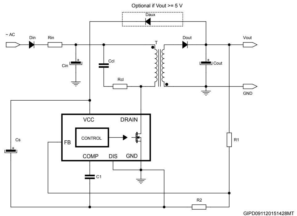
Figure 35. Flyback converter with line OVP (non-isolated)
