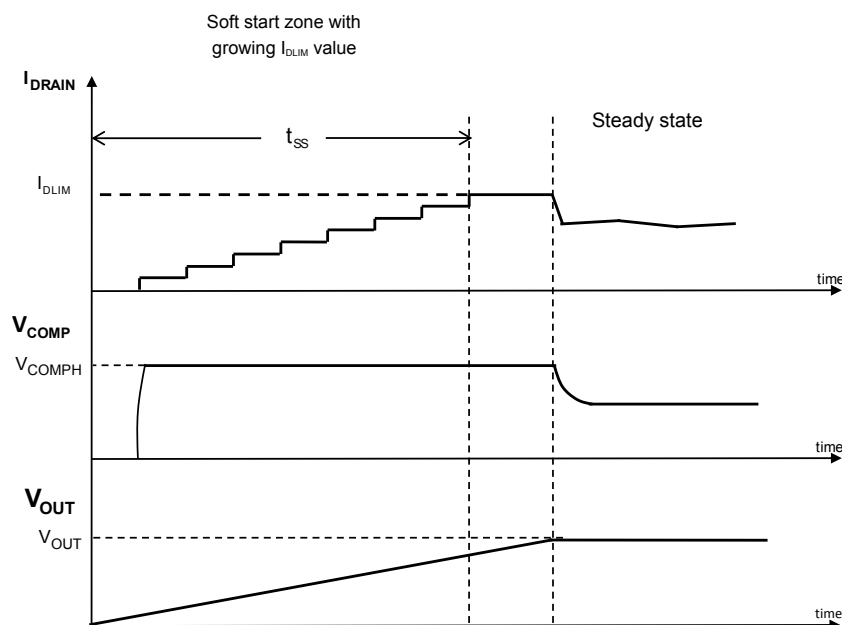
Figure 28. Soft startup
