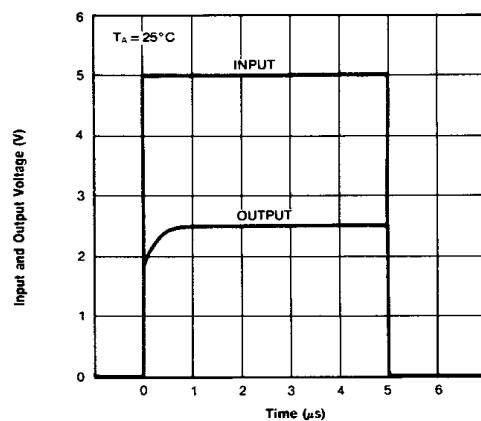
Figure 9. Pulse Response
