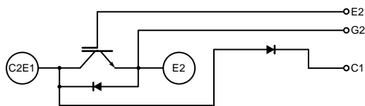
Outline Drawing and Circuit Diagram
