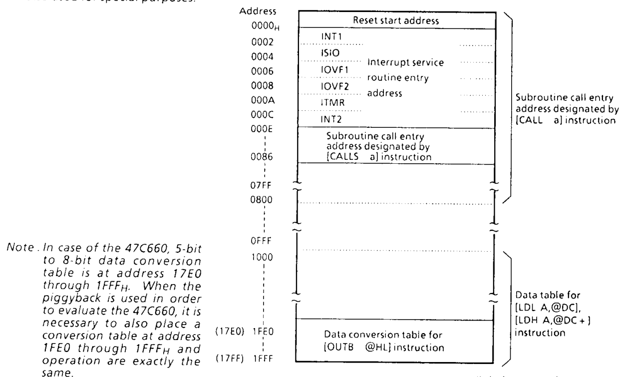
Figure 2-3. Program Memory Map
