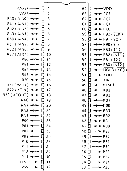
(1) SDIP64
