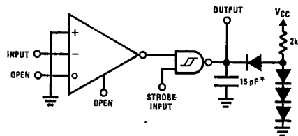
Differential and Strobe Input Signal
