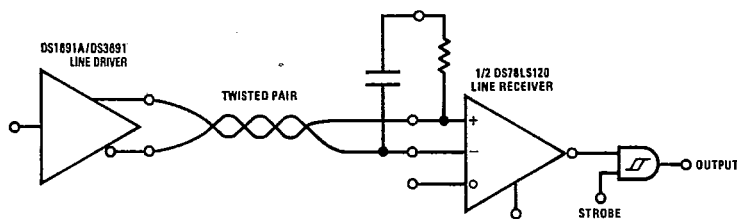
Balanced Data Transmission
