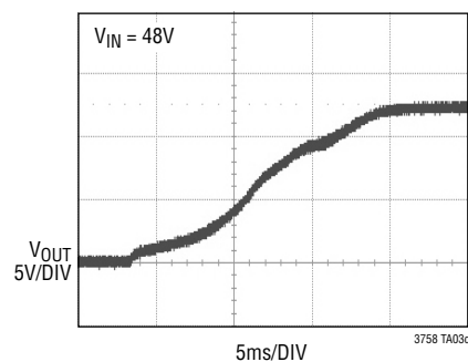
Start-Up Waveform
