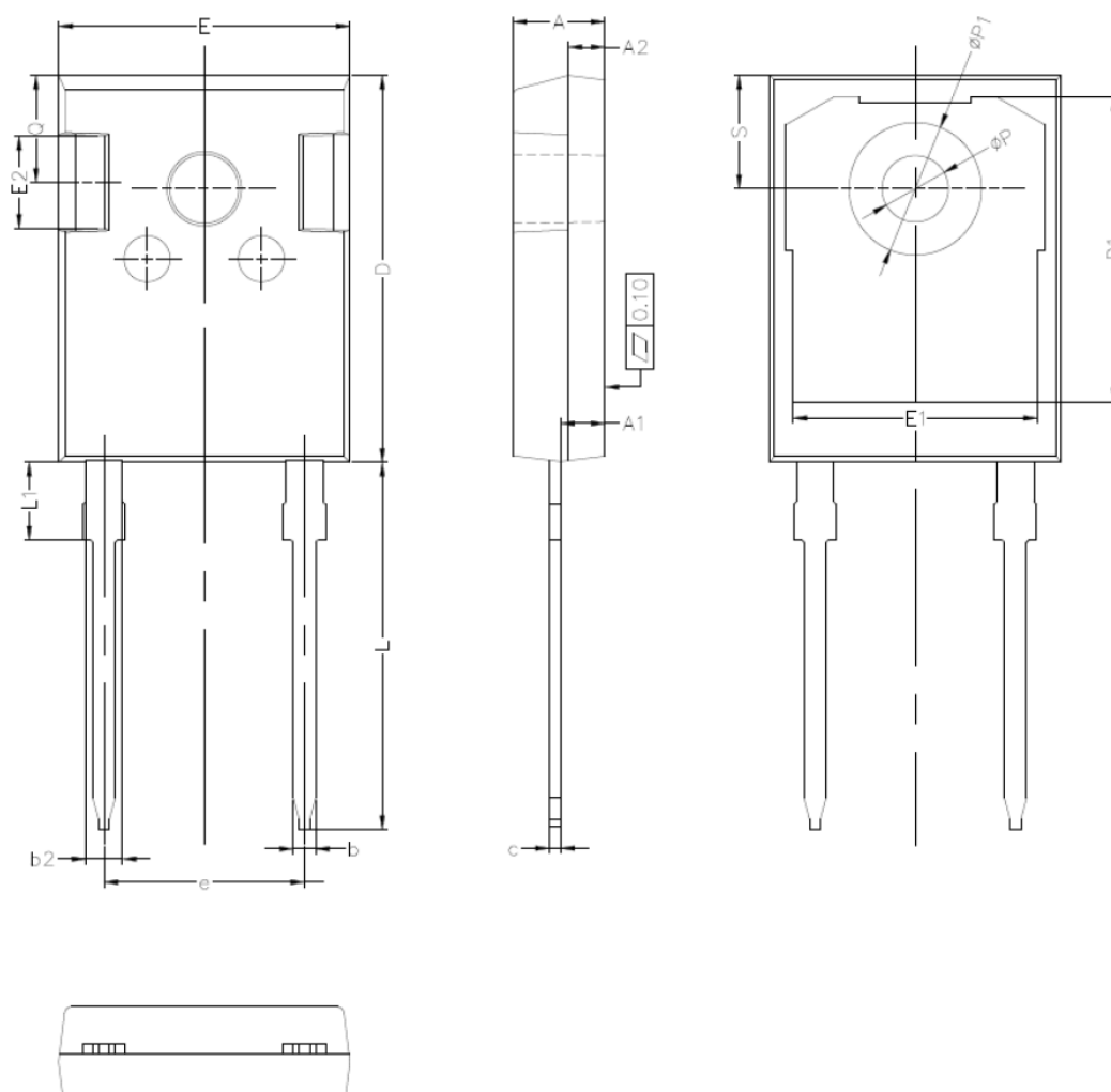
Figure 15. DO-247 LL package outline
