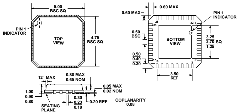
Figure 23. 32-Lead Lead Frame Chip Scale Package [LFCSP] (CP-32) Dimensions shown in millimeters
