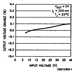
Line Regulation
