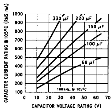
FIGURE 14. RMS Current Ratings for Low ESR Electrolytic Capacitors (Typical)
