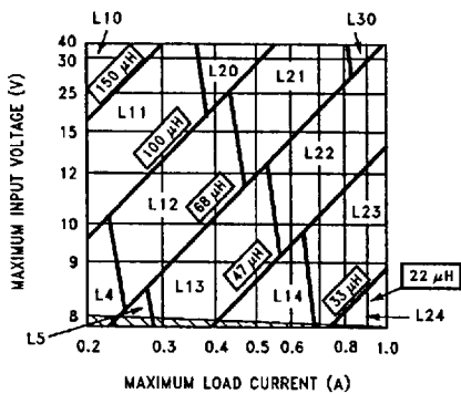
FIGURE 5. LM2675-5.0
