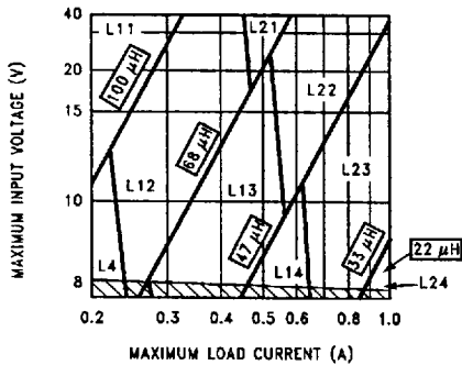
FIGURE 4. LM2675-3.3
