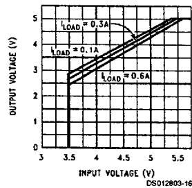
Dropout Voltage—5.0V Option
