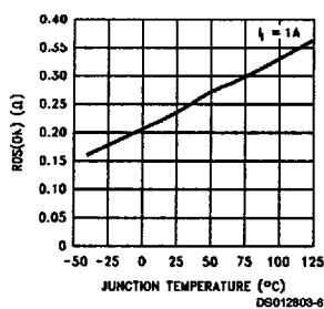
Drain-to-Source Resistance
