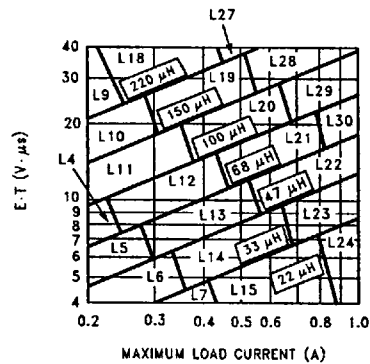
FIGURE 7. LM2675-ADJ
