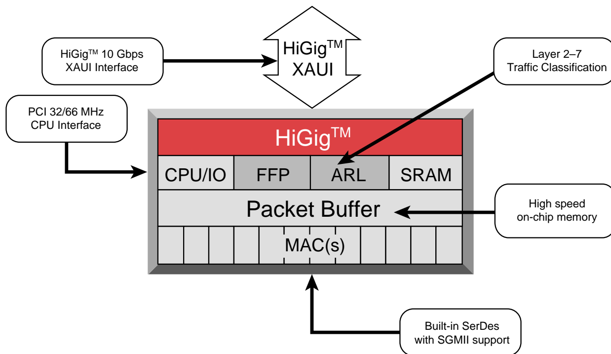
BCM5690 Block Diagram
