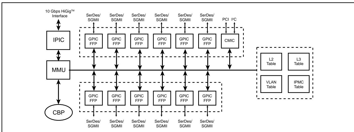
12-Port Gigabit Ethernet Multilayer Switch with HiGig™
