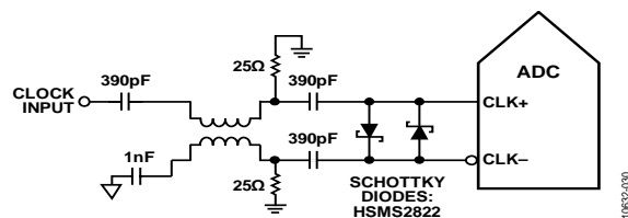
Figure 34. Balun-Coupled Differential Clock (Up to 625 MHz)
