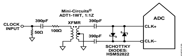
Figure 33. Transformer-Coupled Differential Clock (Up to 200 MHz)
