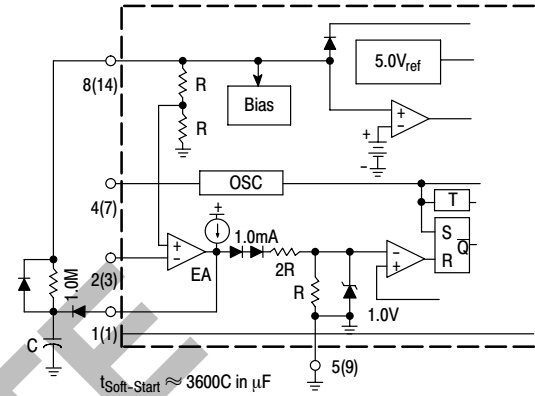
Figure 21. Soft-Start Circuit
