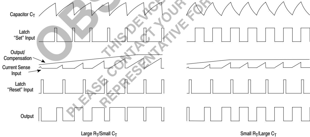
Figure 17. Timing Diagram
