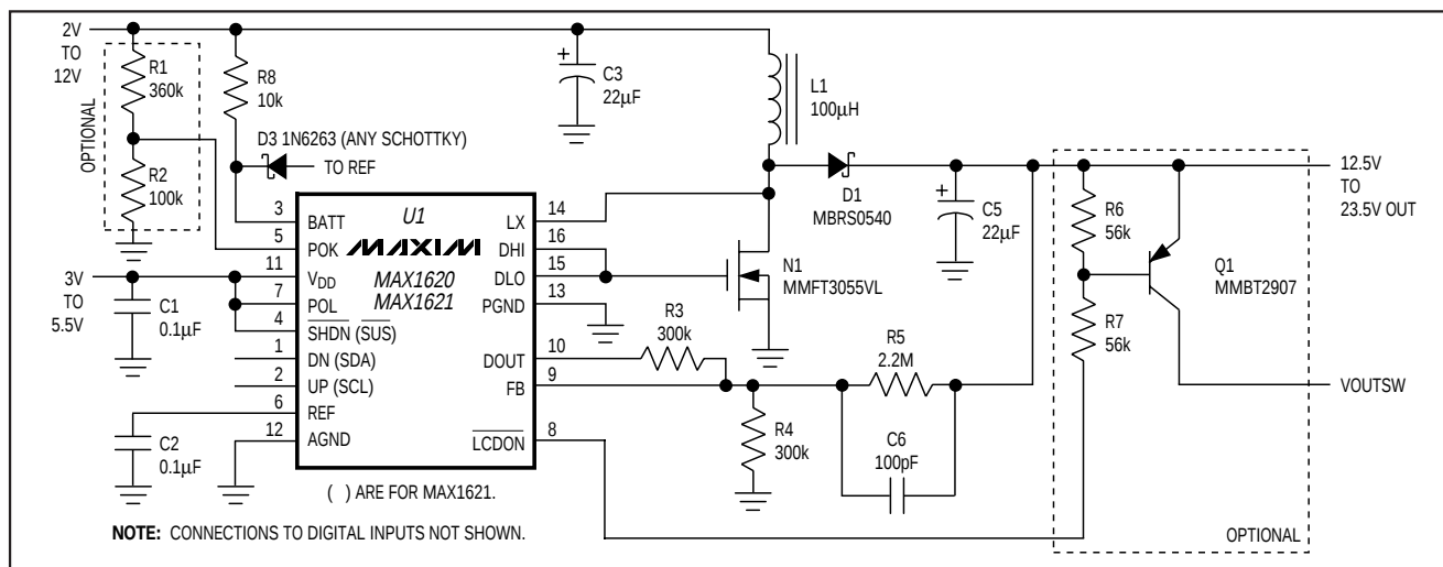
Figure 4. Typical Operating Circuit—Positive Output
