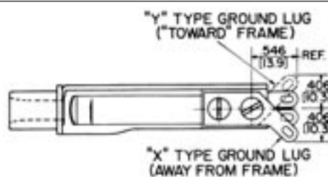
MT-Jax®, Offset Lugs
