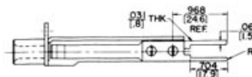
MT-Jax®, Wire-Wrapping Detail
