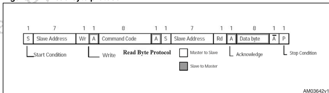
Figure 4. Read byte protocol
