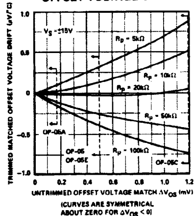
TRIMMED OFFSET VOLTAGE DRIFT
