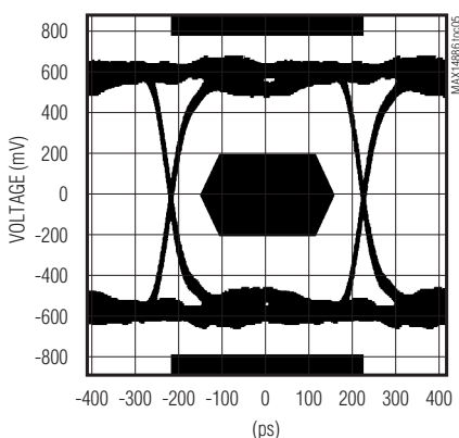
EYE DIAGRAM, V_{IN} = 200mV_{p-p} , 2.25Gbps, 400Ω BACK TERMINATION, R_{SET} = 3k\Omega , FIGURE 1
