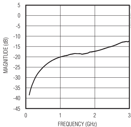
DIFFERENTIAL INPUT RETURN LOSS vs. FREQUENCY
