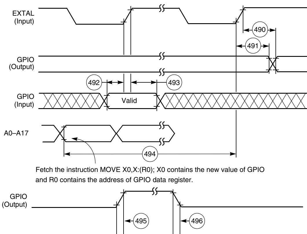
Figure 3-38 GPIO Timing
