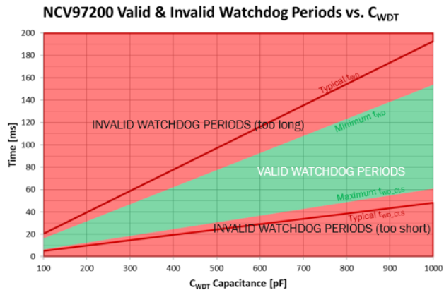
Figure 37. NCV97200 Valid & Invalid Watchdog Periods vs. C_{WDT}
