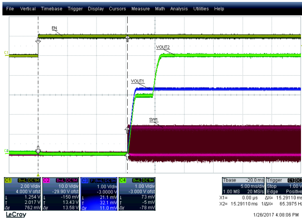
Figure 29. Startup Sequence
