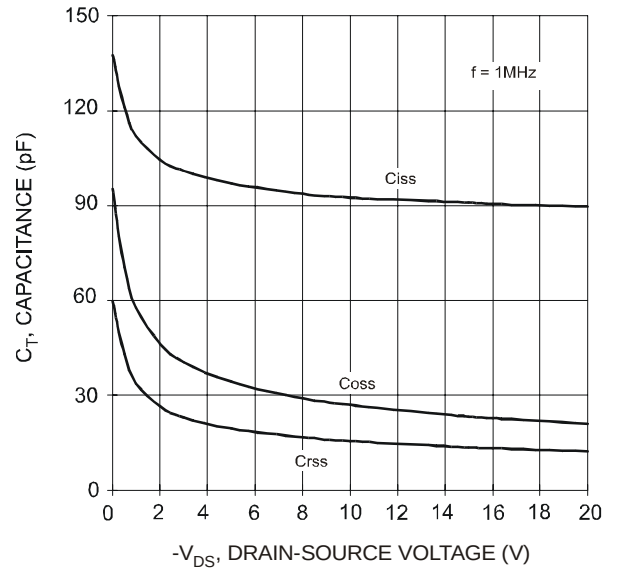
Fig. 20 Typical Capacitance
