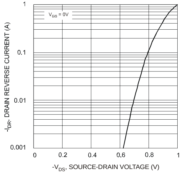
Fig. 18 Reverse Drain Current vs. Source-Drain Voltage
