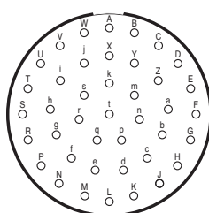
Disposition 20-41 * 41 contacts size 20
