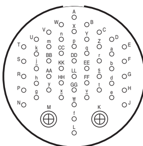
Disposition 24-53 * 51 contacts size 20 2 coax or size 8
