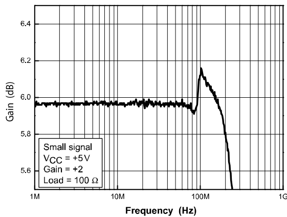
Figure 4: Flatness, gain = 2
