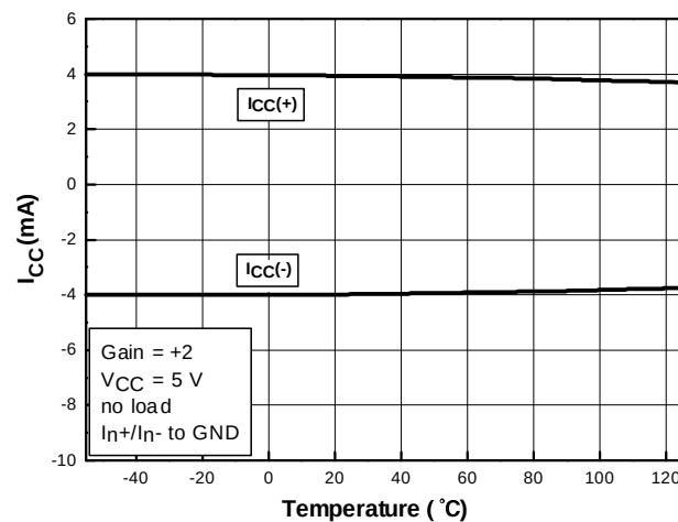
Figure 24: I_{CC} vs. temperature
