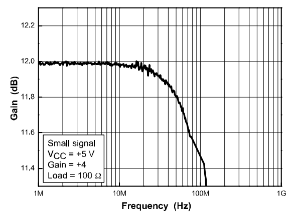
Figure 5: Flatness, gain = 4
