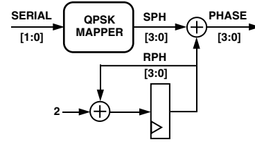
Figure 22. QPSK Mapper
