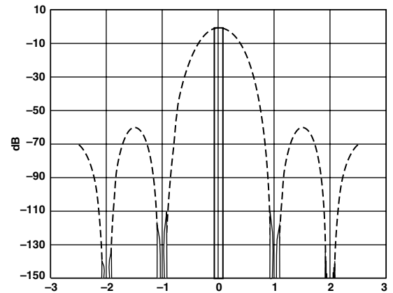
Figure 28. -110 dBc Rejection
