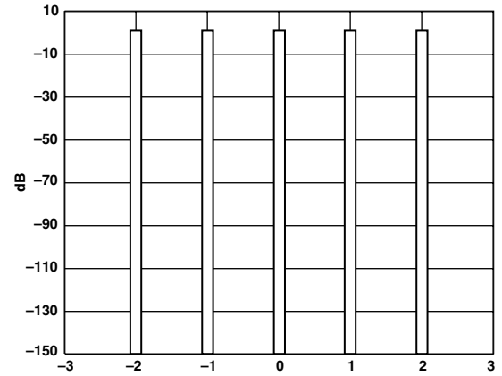
Figure 27. Interpolation Images
