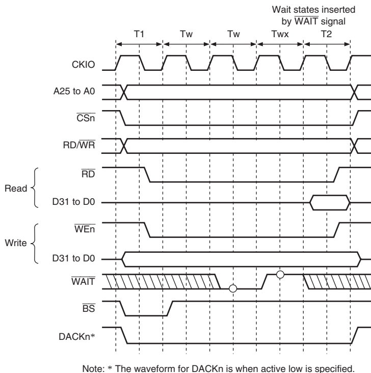
Figure 8.10 Wait Cycle Timing for Normal Space Access (Wait Cycle Insertion Using \overline{\text{WAIT}} Signal)
