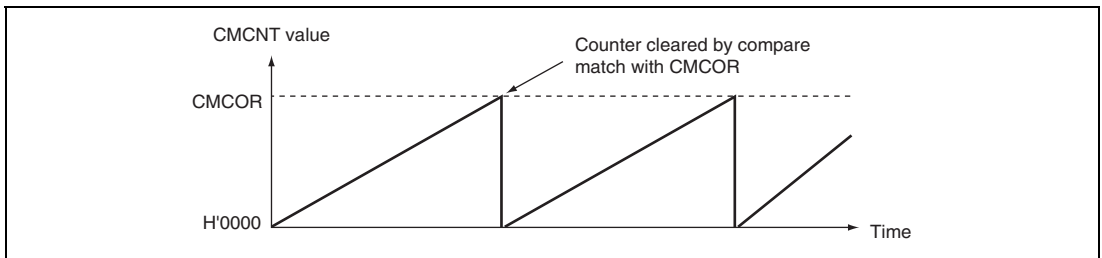
Figure 13.2 Counter Operation
