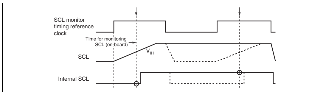
Figure 16.22 Bit Synchronous Circuit Timing
