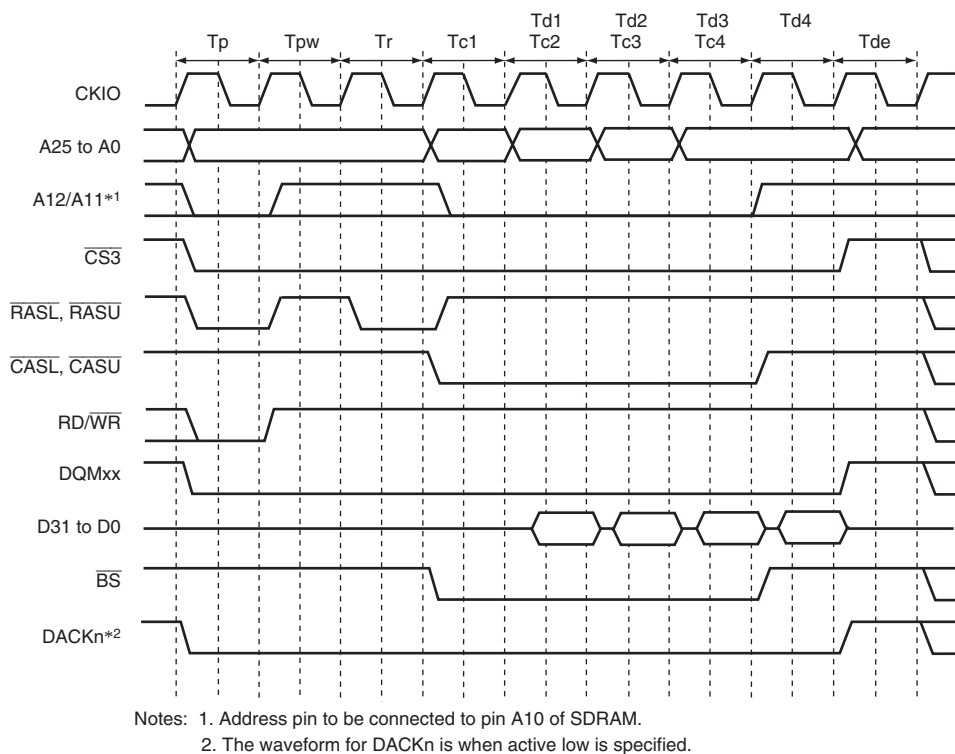
Figure 8.25 Burst Read Timing (Bank Active, Different Row Addresses in the Same Bank, CAS Latency 1)
