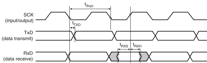
Figure 25.52 SCIF Input/Output Timing in Clocked Synchronous Mode
