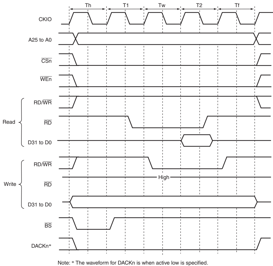
Figure 8.39 Wait Timing for SRAM with Byte Selection (BAS = 1) (SW[1:0] = 01, WR[3:0] = 0001, HW[1:0] = 01)
