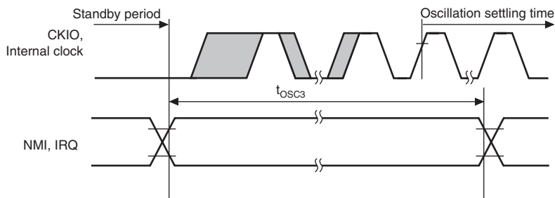
Figure 25.7 Oscillation Settling Time on Return from Standby (Return by NMI or IRQ)
