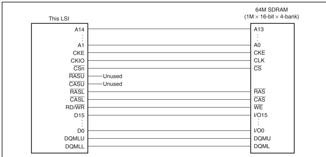
Figure 8.16 Example of 16-Bit Data Width SDRAM Connection ( RASU and CASU are Not Used)
