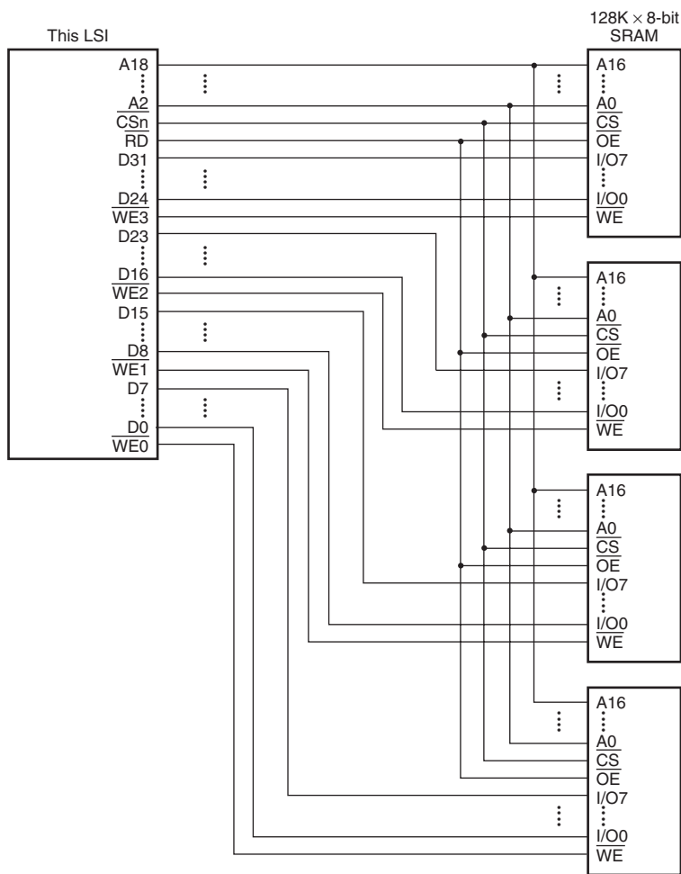
Figure 8.6 Example of 32-Bit Data-Width SRAM Connection
