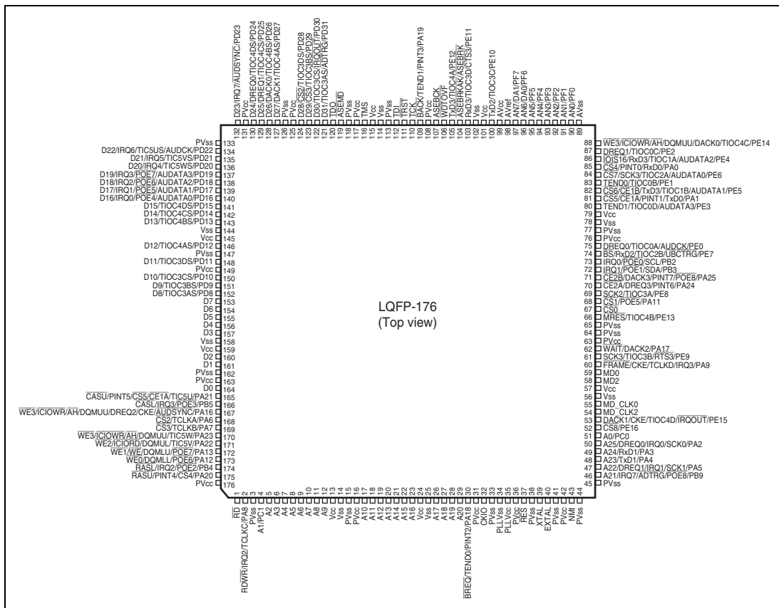
Figure 1.2 Pin Arrangement
