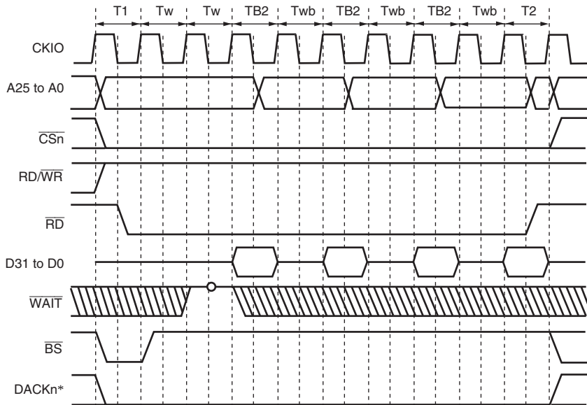
Figure 8.36 Burst ROM Access Timing (Clocked Asynchronous) (Bus Width = 32 Bits, 16-Byte Transfer (Number of Burst 4), Wait Cycles Inserted in First Access = 2, Wait Cycles Inserted in Second and Subsequent Access Cycles = 1)
