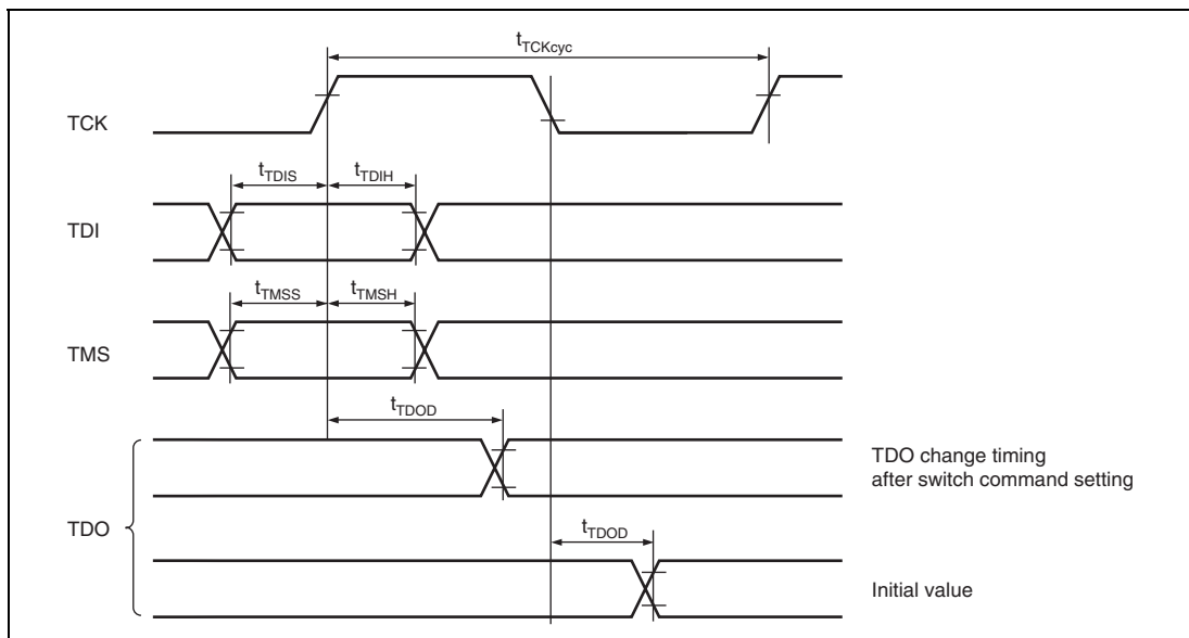
Figure 25.57 H-UDI Data Transfer Timing
