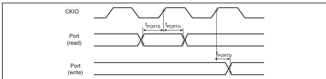
Figure 25.55 I/O Port Timing
