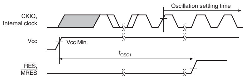
Figure 25.5 Power-On Oscillation Settling Time
