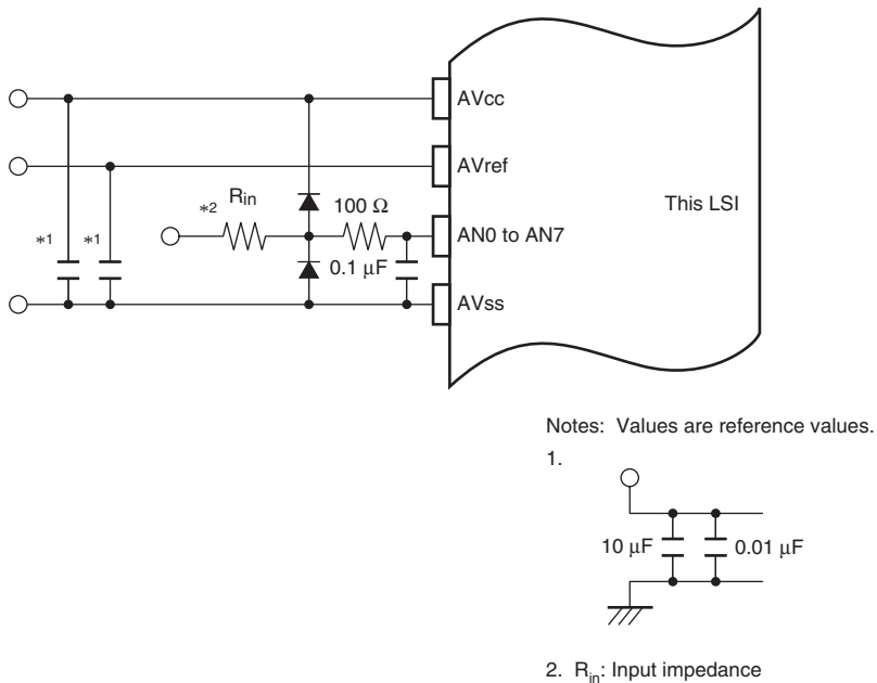
Figure 17.8 Example of Analog Input Protection Circuit
