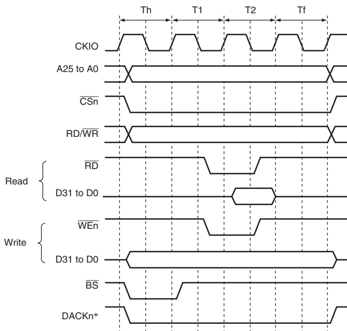
Figure 8.11 \overline{\text{CSn}} Assert Period Expansion
