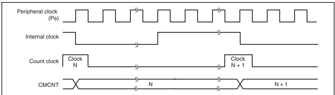
Figure 13.3 Count Timing
