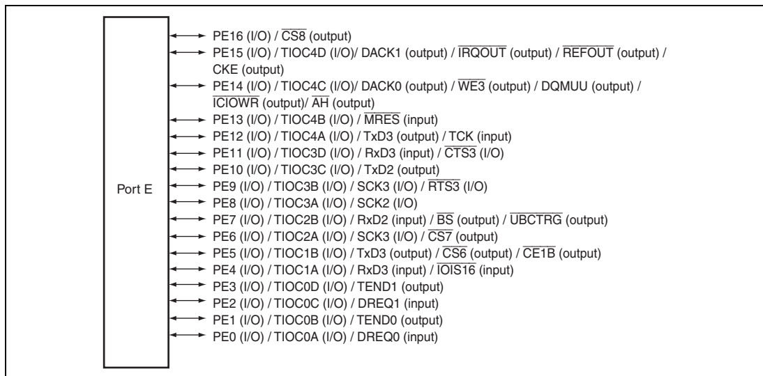
Figure 20.5 Port E
