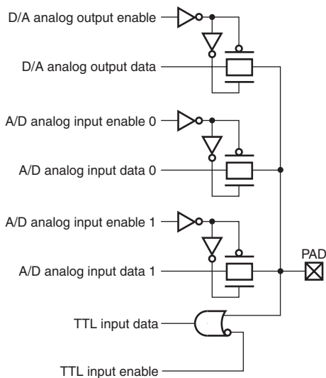
Figure 1.18 Simplified Circuit Diagram (TTL OR Input, Common Buffer for A/D 2-Channel Input and D/A Output)
