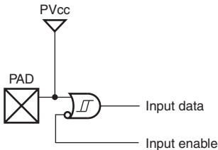
Figure 1.6 Simplified Circuit Diagram (Schmitt OR Input Buffer with Pull-up)
