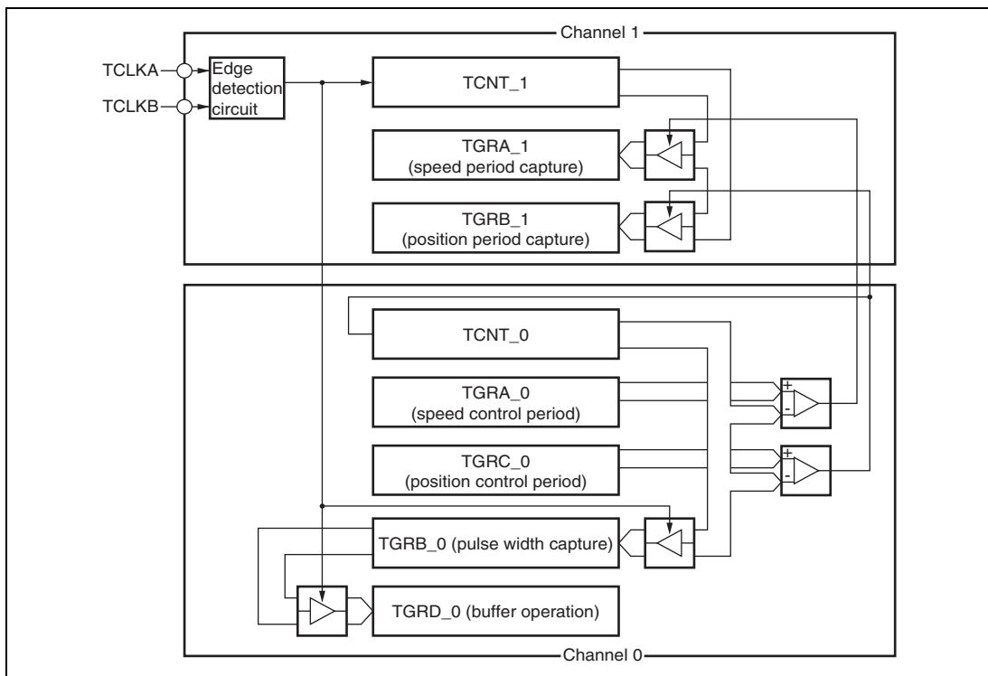
Figure 10.34 Phase Counting Mode Application Example
