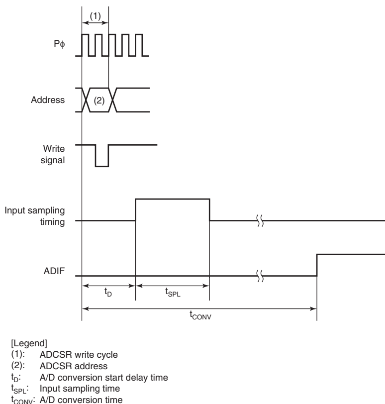
Figure 17.5 A/D Conversion Timing
