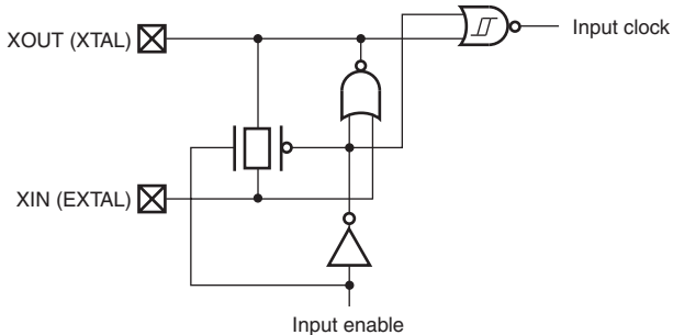
Figure 1.3 Simplified Circuit Diagram (Oscillation Buffer)
