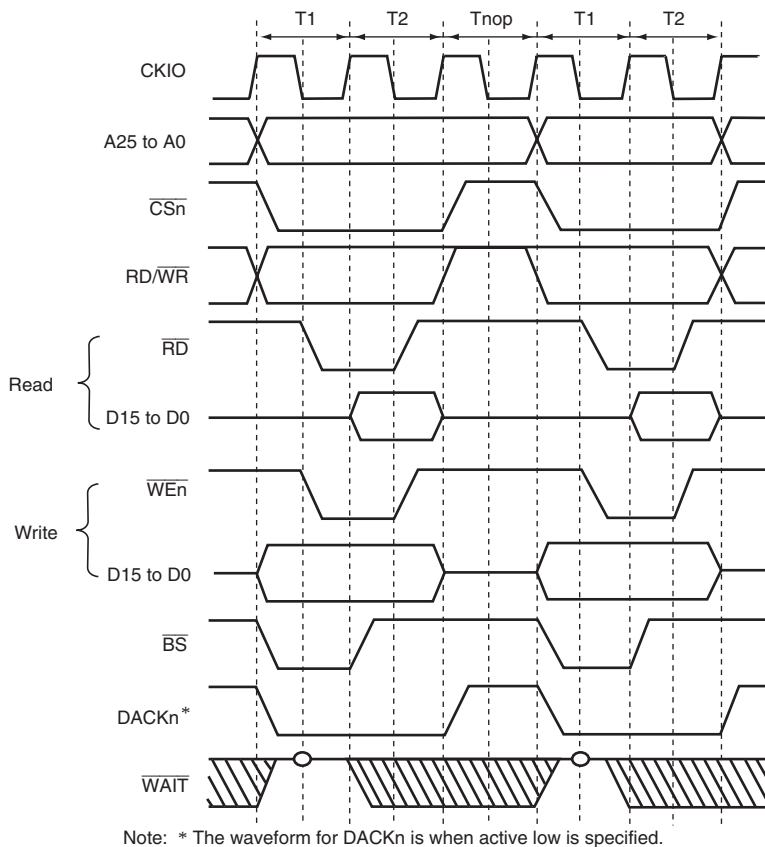
Figure 8.4 Continuous Access for Normal Space 1 Bus Width = 16 Bits, Longword Access, CSnWCR.WM Bit = 0 (Access Wait = 0, Cycle Wait = 0)
