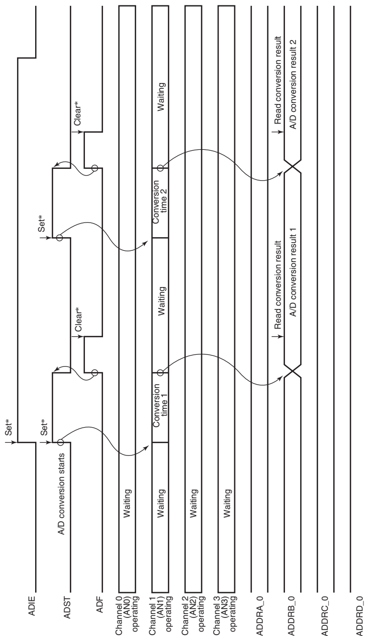
Figure 17.2 Example of A/D Converter Operation (Single Mode, One Channel Selected)
