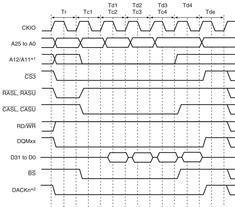
Figure 8.23 Burst Read Timing (Bank Active, Different Bank, CAS Latency 1)
