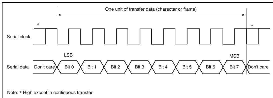
Figure 15.11 Data Format in Clocked Synchronous Communication
