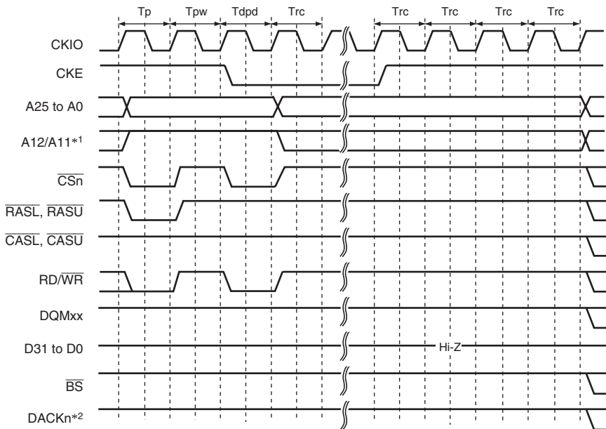
Figure 8.35 Deep Power-Down Mode Transition Timing
