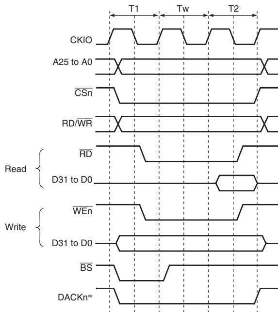
Figure 8.9 Wait Timing for Normal Space Access (Software Wait Only)
