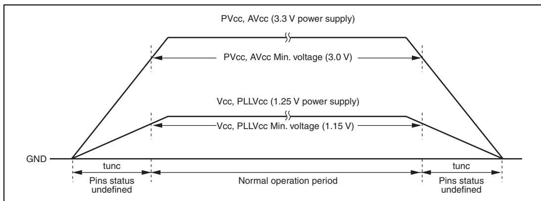
Figure 25.1 Power-on/Power-off Sequence
