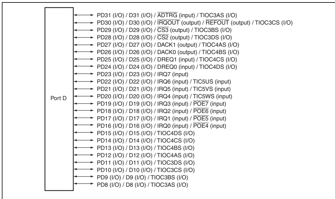
Figure 20.4 Port D
