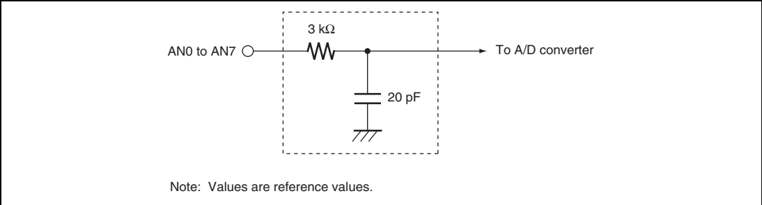
Figure 17.9 Analog Input Pin Equivalent Circuit
