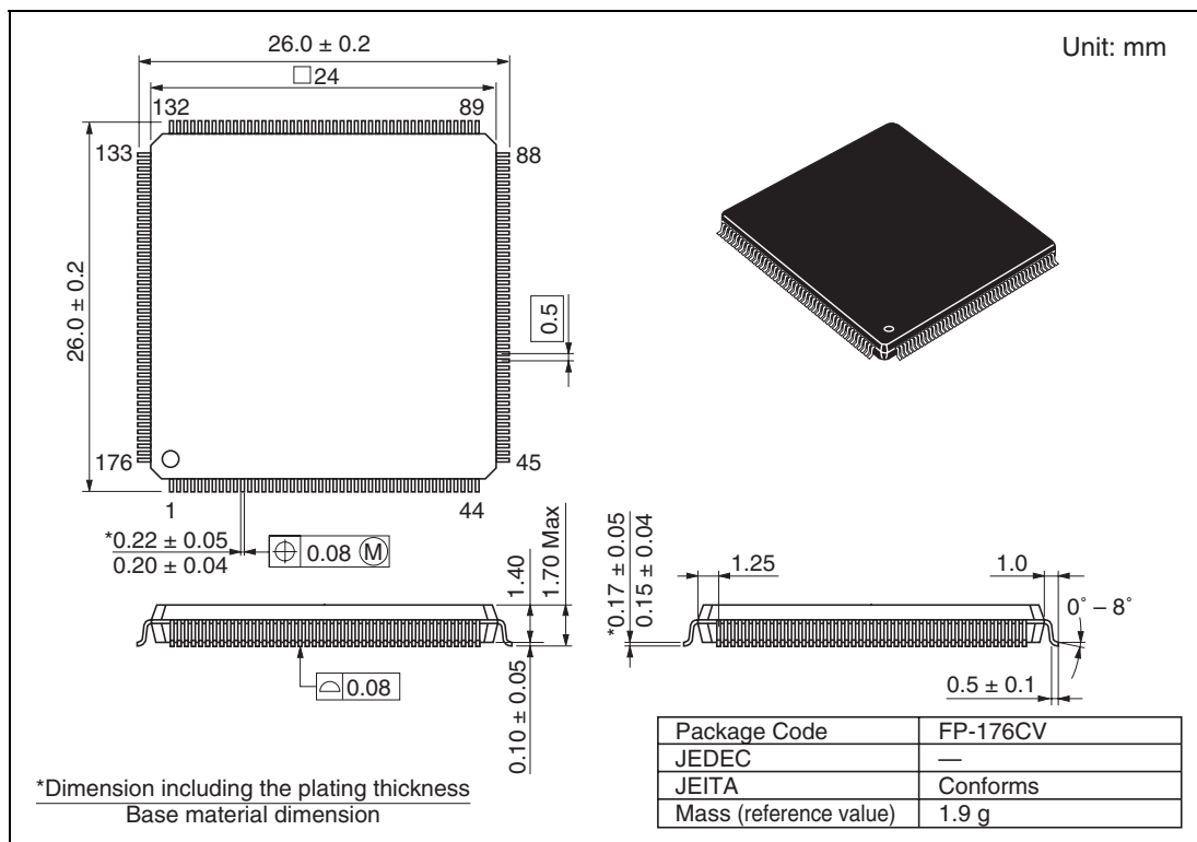
Figure C.1 Package Dimensions
