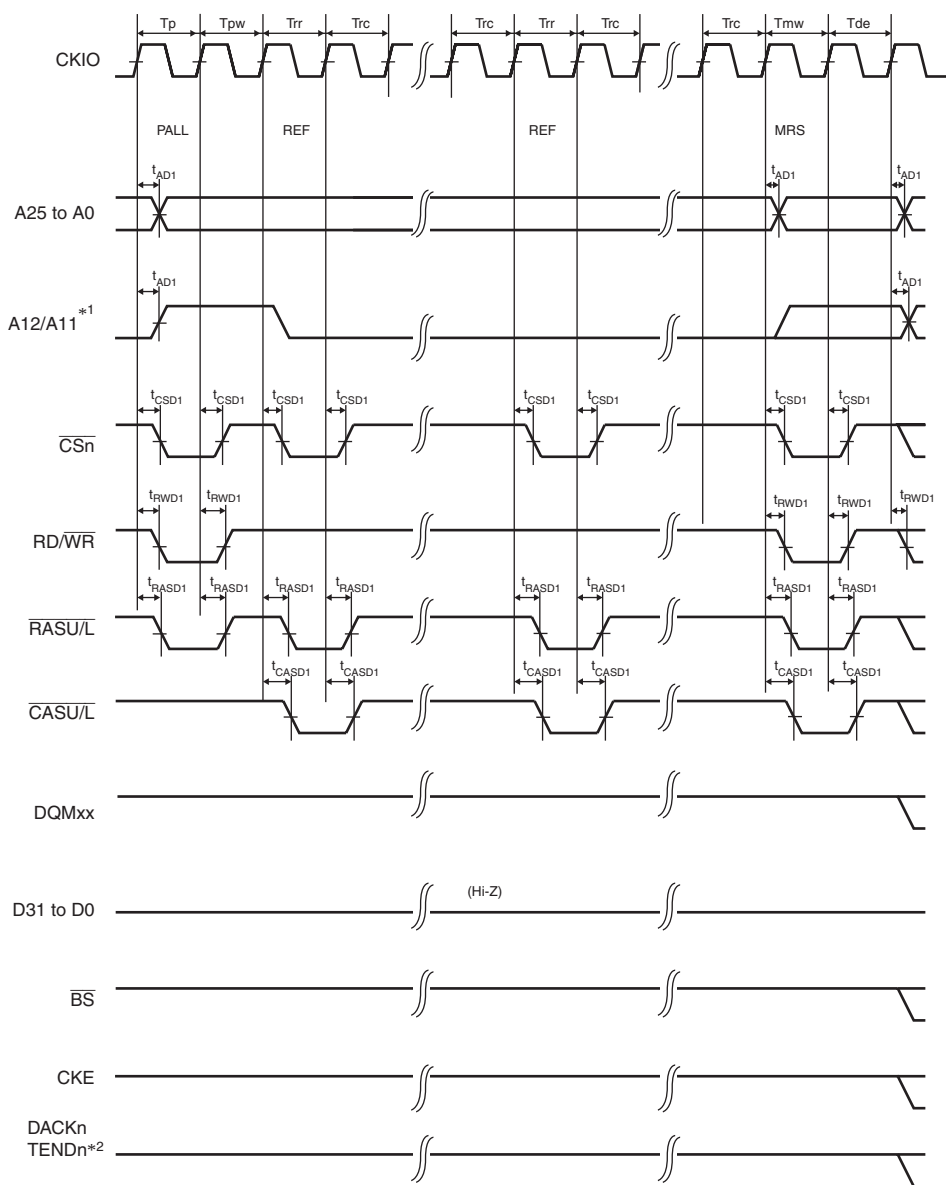
Figure 25.37 Synchronous DRAM Mode Register Write Timing (WTRP = 1 Cycle)
