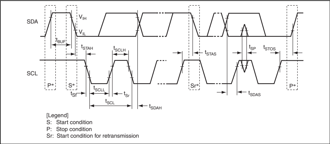
Figure 25.53 I²C Bus Interface 3 Input/Output Timing
