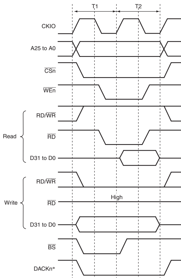
Figure 8.37 Basic Access Timing for SRAM with Byte Selection (BAS = 0)
