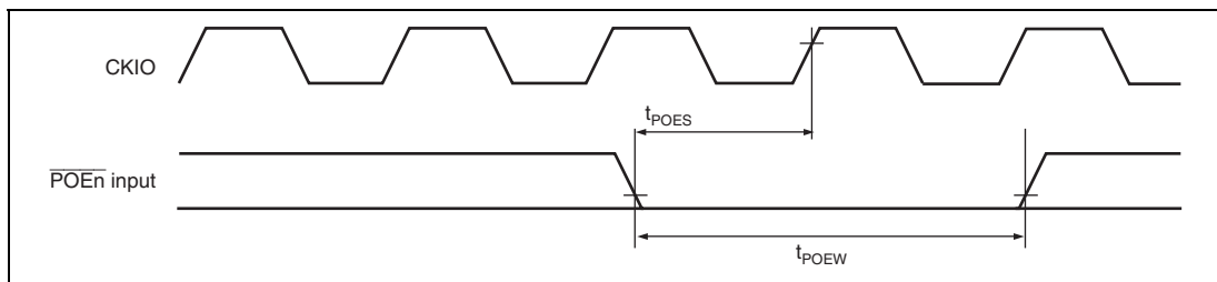
Figure 25.49 POE2 Input/Output Timing
