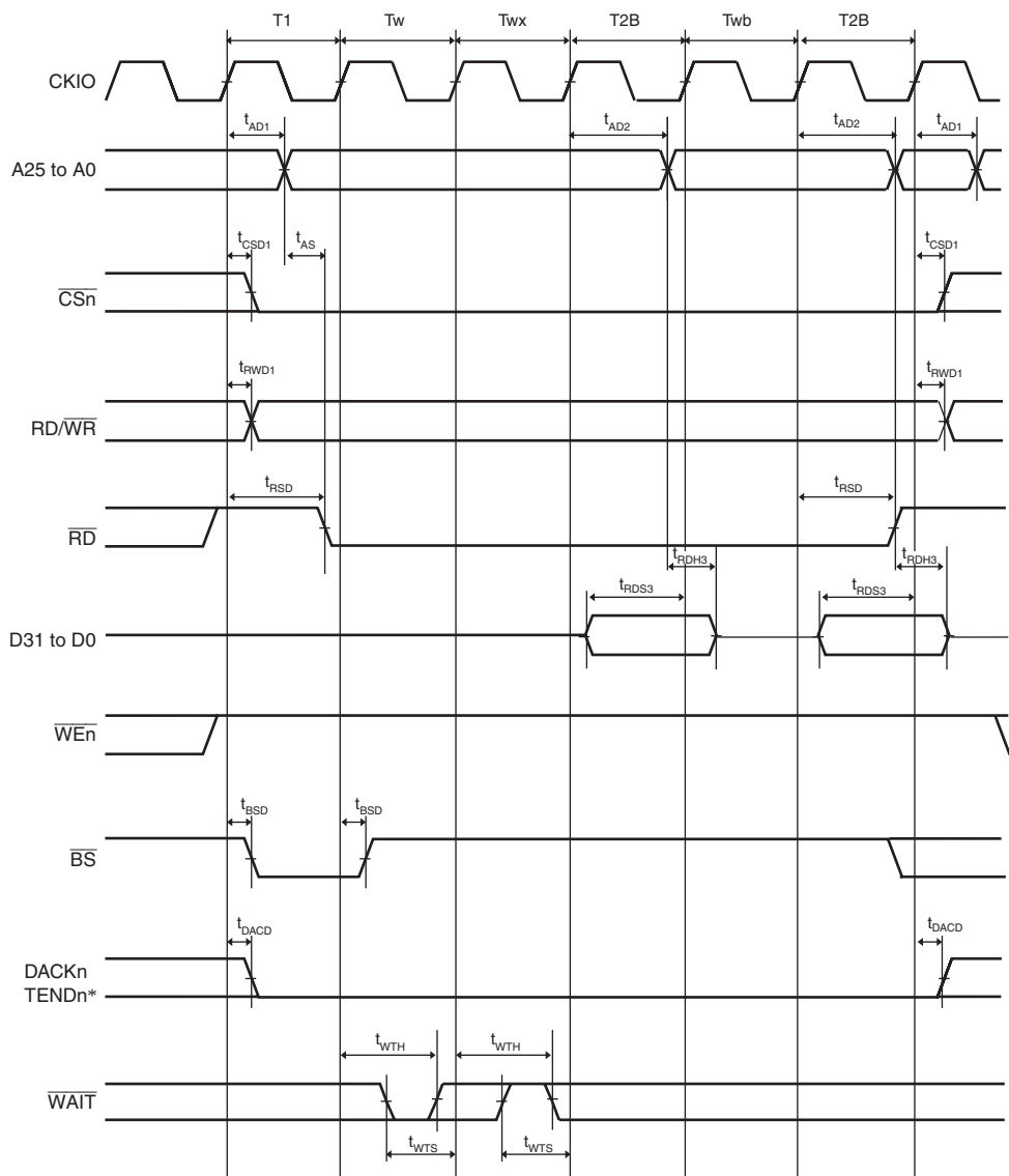
Figure 25.20 Burst ROM Read Cycle (One Software Wait Cycle, One Asynchronous External Burst Wait Cycle, Two Burst)
