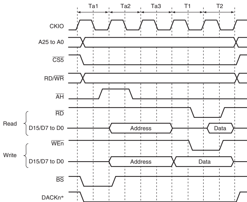
Figure 8.12 Access Timing for MPX Space (Address Cycle No Wait, Data Cycle No Wait)
