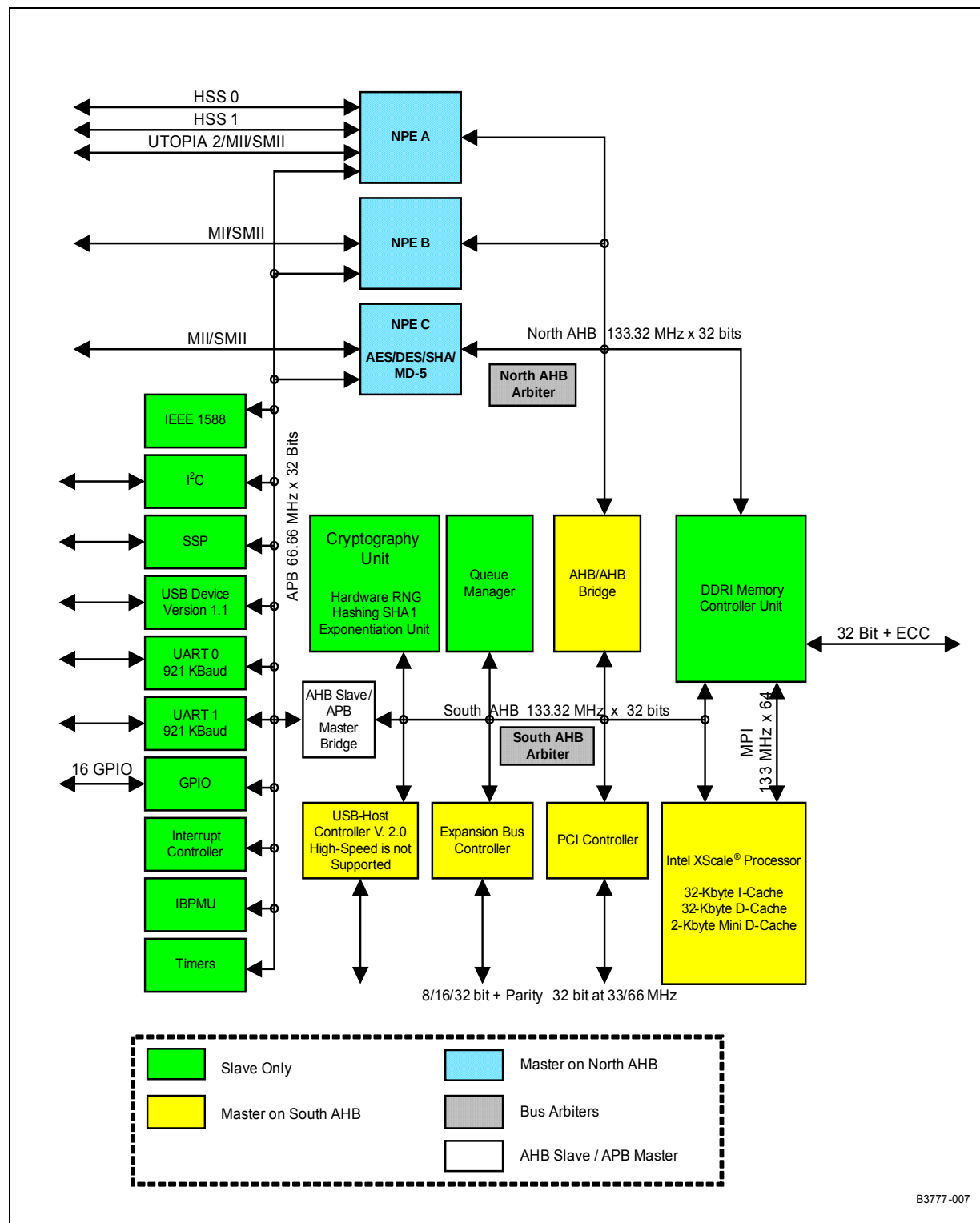
Figure 1. Intel® IXP465 Network Processor Block Diagram
