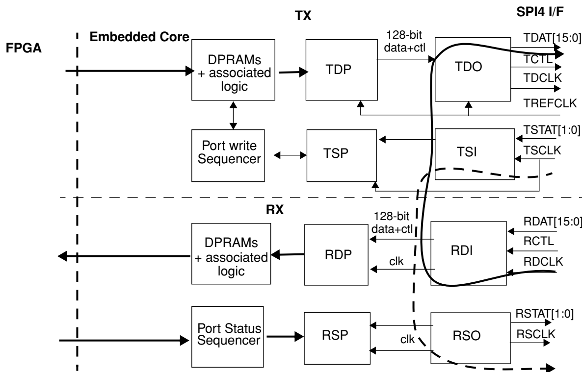
Figure 43. Far End Loopback
