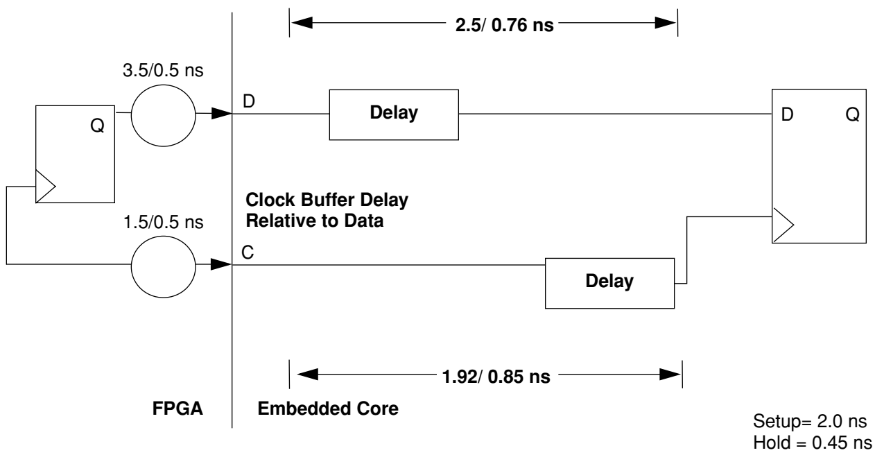
Figure 82. F_MC_RDFIFO_RE, F_MC_RIFIFO_WE Clock: F_MC_RCLK
