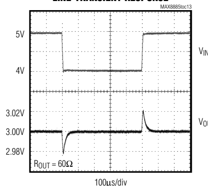
LINE-TRANSIENT RESPONSE
