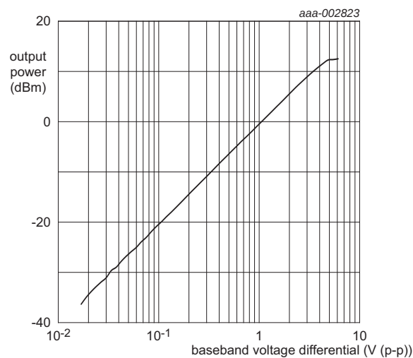
Fig 12. P_o versus baseband voltage at 2140 MHz
